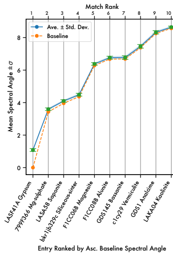
LASF41A Gypsum Mean Spectral Angle Match
