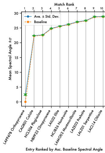
LAPP47B Orthopyroxene Mean Spectral Angle Match
