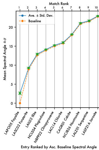
LAPO05 Fayalite Mean Spectral Angle Match
