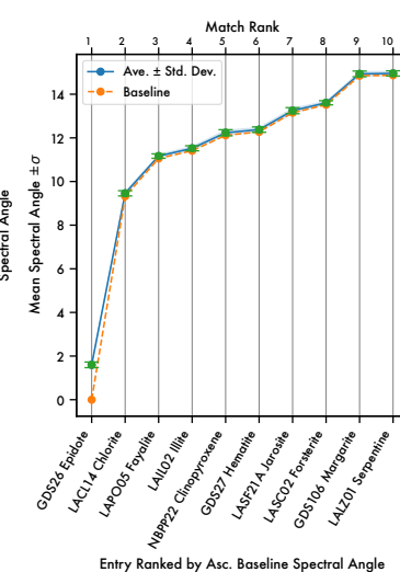
GDS26 Epidote Mean Spectral Angle Match
