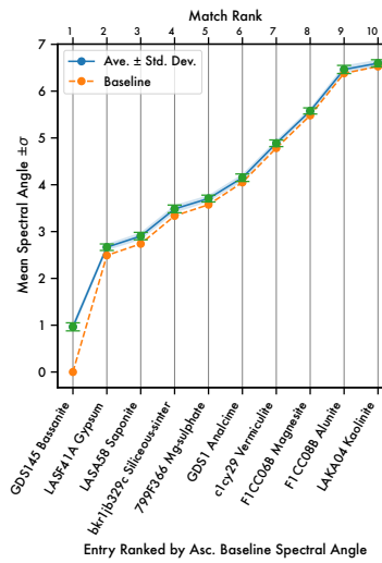
GDS145 Bassanite Mean Spectral Angle Match
