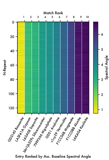
GDS145 Bassanite Mean Spectral Angle Match
